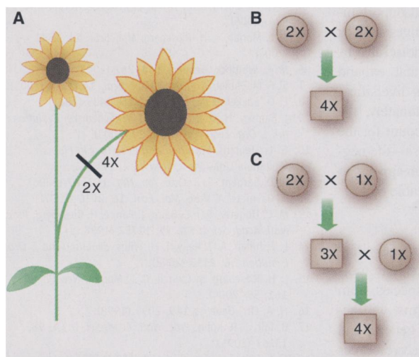
Fig. 3. Mechanisms by which polyploids can arise. (A) Somatic doubling, in which chromosome number is doubled in vegetative tissue that gives rise to reproductive organs. (B) Fusion of unreduced gametes that are produced when cell walls fail to form in the final stage of meiosis. (C) A triploid bridge, in which unreduced and reduced gametes form triploids. If the triploids also produce unreduced gametes, the triploid gametes may fuse with reduced gametes from diploid individuals to generate stable tetraploids.
