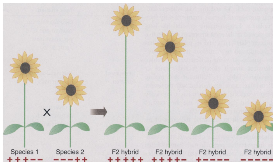
Fig. 2. Genetic basis of transgressive segregation showing how segregating hybrids can combine plus and minus alleles from parental species, thereby generating extreme phenotypes or adaptations to extreme habitats.
